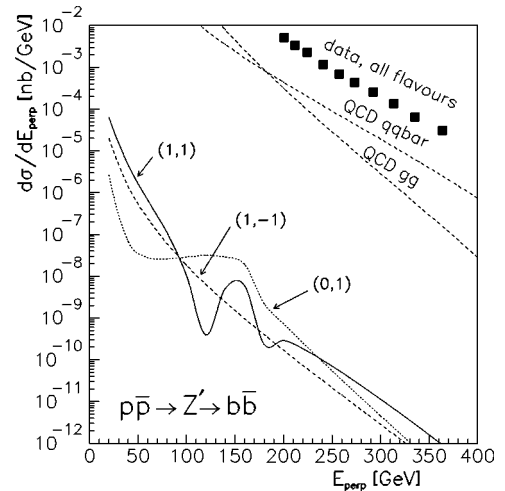
FIG. 3. Similar to Fig. 2, but for M_{Z'} = 200 GeV only. Three cases of q\bar{q}Z' couplings are considered: (g_{Z'} a'_t, g_{Z'} a'_b) = (1,1) (solid line), (0,1) (dotted line), and (1,-1) (dashed line).
