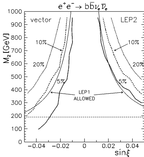
FIG. 11. Bounds anticipated from LEP2 for e^+e^- \rightarrow b\bar{b}\nu_e\bar{\nu}_e at levels of assumed precision as indicated by the labels. Also shown is the allowed region of \sin\xi and M_2 obtained from LEP1 data (95% C.L.) for the process e^+e^- \rightarrow b\bar{b} .
