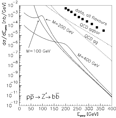
FIG. 1. Cross sections for inclusive jet production at the Tevatron, p\bar{p} collisions at E_{c.m.}=1.8 TeV. The solid curves represent Drell–Yan-type production of Z' , from b and \bar{b} (sea) quarks in the initial state. Three masses are considered, M_{Z'}=100, 200 and 400 GeV. The couplings are g_{Z'}v'_b=g_{Z'}a'_b=1 . Also the contributions from the dominant QCD mechanisms are shown, as well as data (summed over all flavors) [26].
