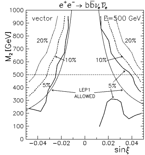
FIG. 12. Bounds anticipated from \sqrt{s}=500 GeV for e^+e^- \rightarrow b\bar{b}\nu_e\bar{\nu}_e at levels of assumed precision as indicated by the labels. Also shown is the allowed region of \sin\xi and M_2 obtained from LEP1 data (95% C.L.) for the process e^+e^- \rightarrow b\bar{b} .
