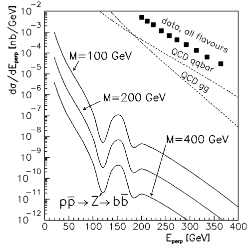
FIG. 2. Cross sections for inclusive jet production at the Tevatron, p\bar{p} collisions at E_{c.m.} = 1.8 TeV. The solid curves represent production of Z' , from gluon fusion. Three masses are considered, M_{Z'} = 100, 200 and 400 GeV. Both b and t quarks contribute to the triangle diagram, with equal couplings, g_{Z'} a'_b = g_{Z'} a'_t = 1 . Also the contributions from the dominant QCD mechanisms are shown, as well as data (summed over all flavors) [26].
